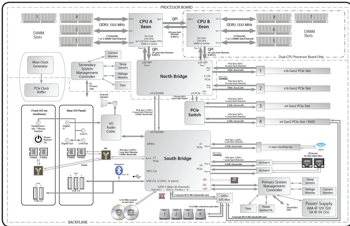
Image courtesy Apple Computer, Inc. Figure 4-3: Mac Pro Main Logic Board Block Diagram
