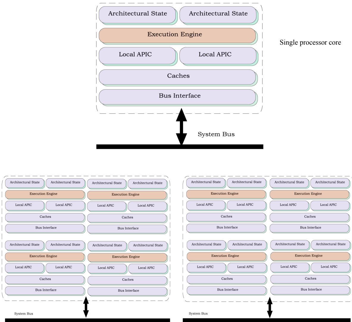
Figure 4-5: Two Intel Xeon 5520 Quad Core Microprocessors
