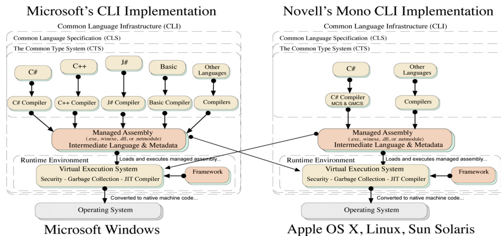
Figure 4-17: Managed Assemblies can be Executed on any System that Implements the Common Language Infrastructure
